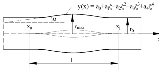
Figure 3: Patch geometry
