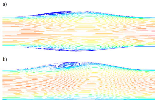
Figure 8: Dilation of the artery: a) symmetric b) asymmetric.
