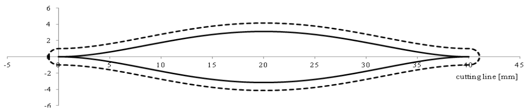
Figure 13: Patch outline with overlap on the stitching (external profile) and without overlap on the stitching (internal profile), for the cutting length l = 40 mm, the width of the overlap on the suture s = 1 mm
