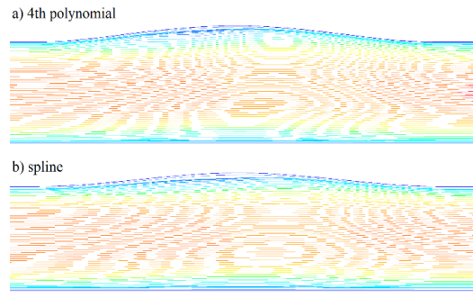
Figure 9: Comparison of geometries: a) fourth degree polynomial b) third degree polynomial spline.
