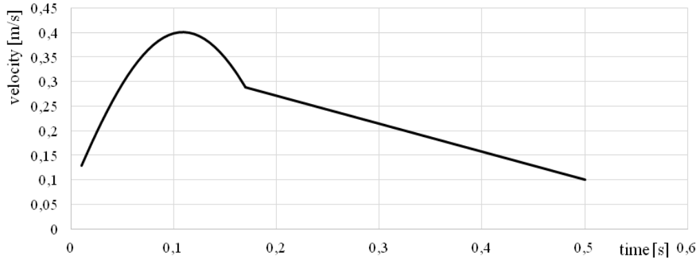
Figure 7: Inlet velocity profile (one pulse duration = 0.5 s)
