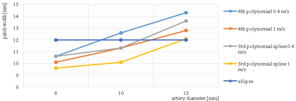
Figure 12: Limit width of the patch depending on the diameter of the artery (velocity 0.4 m/s; 1 m/s).
