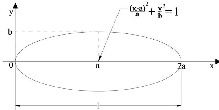
Figure 5: Elliptical patch
