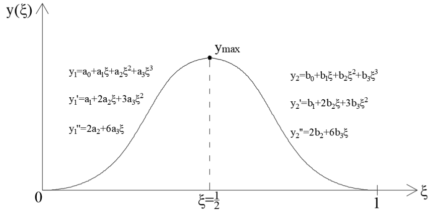
Figure 4: Analytical description of the spline function
