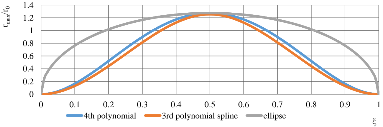
Figure 6: Comparison of patch geometries
